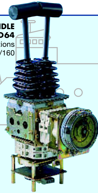
MULTI-AXIS CONTROLLER V6 Explosion protected (flame proof) applications Catalog 1/104
